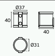
IN.09.005.1.TCO Conector / Connector / Conector
