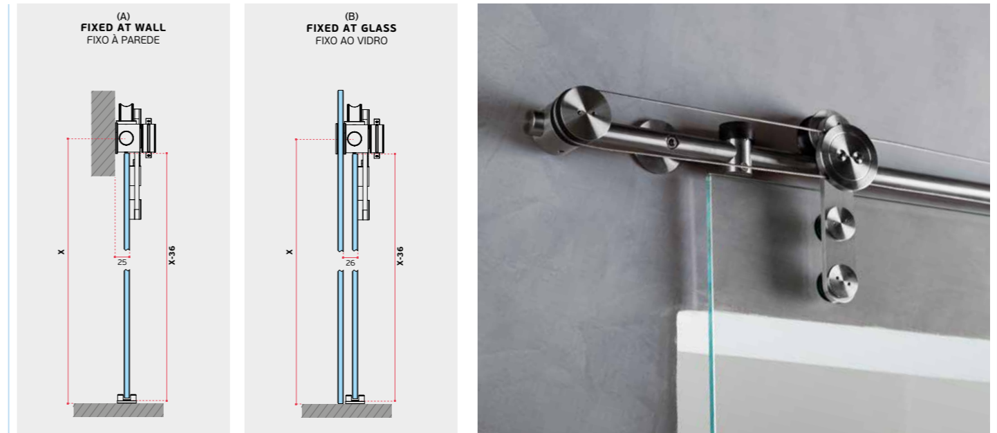
(A) FIXO À PAREDE / FIXED AT WALL / FIJADO A PARED
