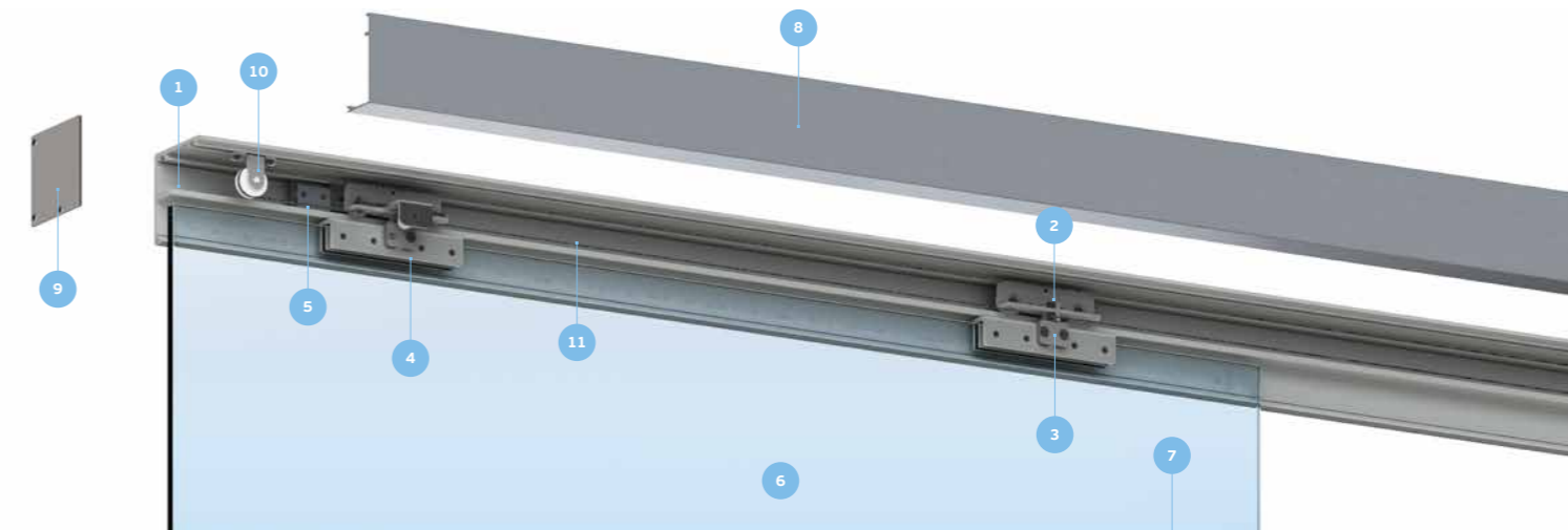
(A) FIXO À PAREDE / FIXED AT WALL / FIJADO A LA PARED.
