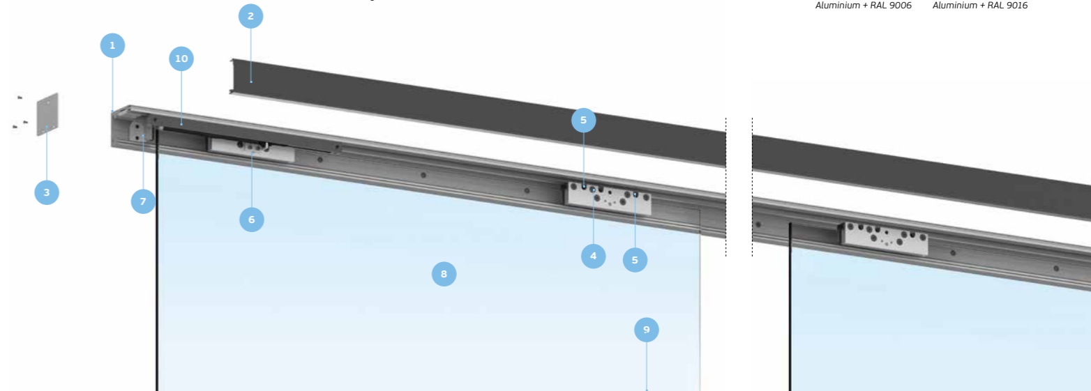
(A) FIXO À PAREDE / FIXED AT WALL / FIJADO A LA PARED.
