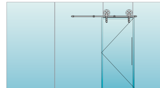
(B) FIXO AO VIDRO / FIXED AT GLASS / FIJA EN CRISTAL CARRIL / RAIL 1900mm
