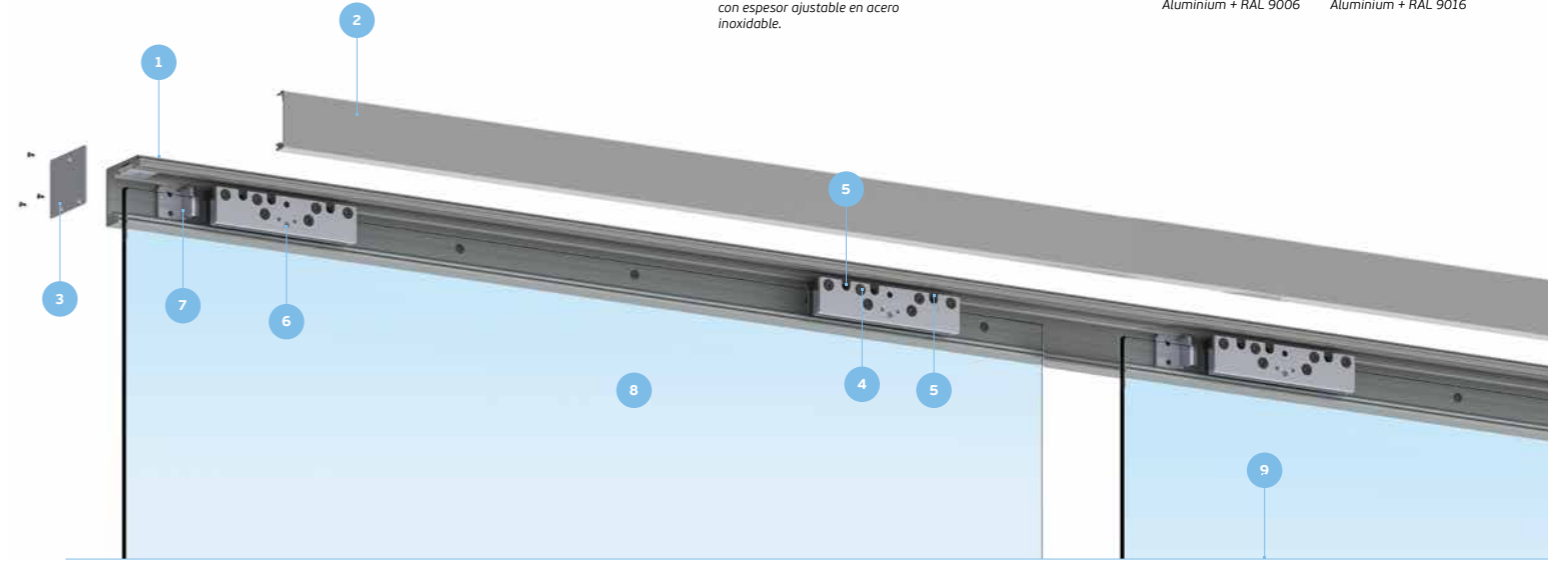
(A) FIXO À PAREDE / FIXED AT WALL / FIJADO A LA PARED.
